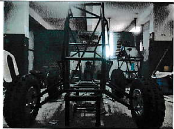
Photograph 2: Fabrication of Rollcage of ATV inside the WORKSHOP
